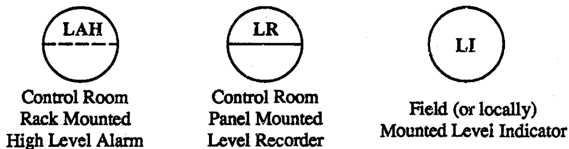
Figure 2: ISA Symbols and the Instruments they Represent.
